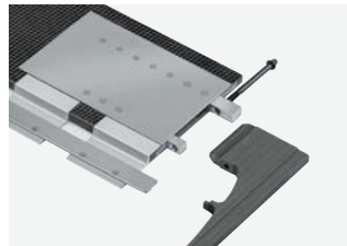
litespeed® Carbon corner connection
